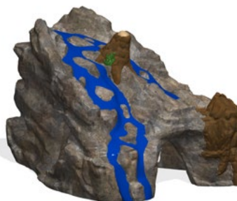
Water Rock
